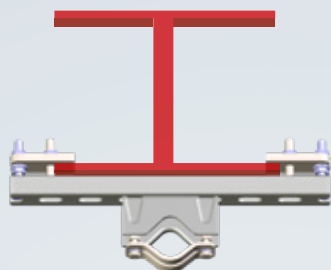
Example: H-carrier fastening
