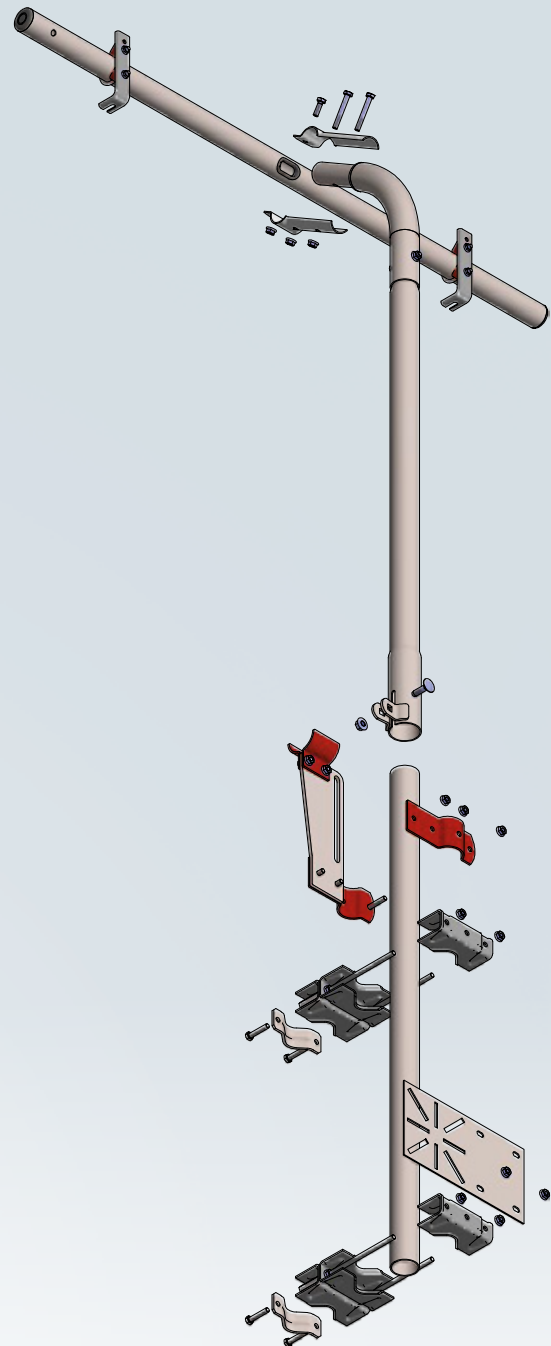
Example: Railing mast system 120° with safety module - folding device
